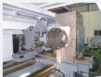
Driving tool with Y axis + spindle with CS / CF (option) is available.
