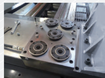
Quick change system for turning / boring bar / milling head / grinding attachment.
