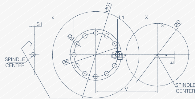
POWER TURRET VDI AXIAL MOUNTING OPT TC-50L22 ~ TC-50L72
