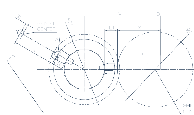
POWER TURRET BMT AXIAL RADIAL MOUNTING OPT
