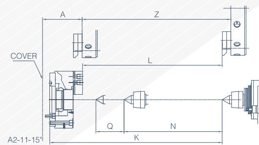
POWER TURRET VDI AXIAL MOUNTING OPT TC-50L22 ~ TC-50L72
