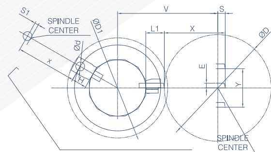
POWER TURRET VDI AXIAL RADIAL MOUNTING OPT.
