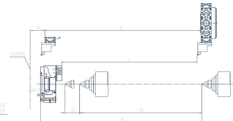
POWER TURRET BMT AXIAL RADIAL MOUNTING OPT
