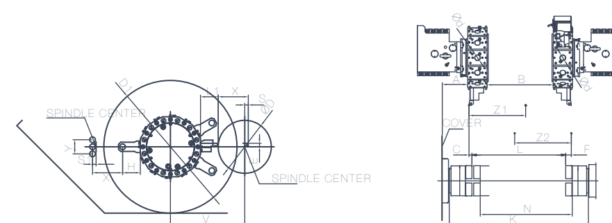
POWER TURRET / TWIN SPINDLE / TWIN TURRET / Y AXIS VDI RADIAL MOUNTING OPT.
