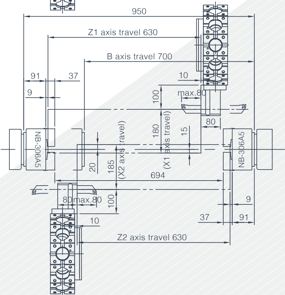
ID Tool Holder
