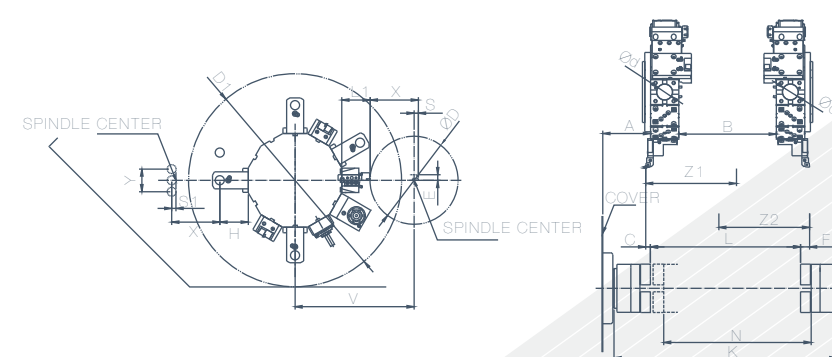
POWER TURRET / TWIN SPINDLE / TWIN TURRET / Y AXIS BMT RADIAL MOUNTING OPT.
