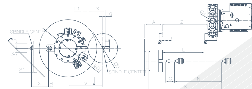
POWER TURRET / Y AXIS BMT RADIAL MOUNTING OPT.
