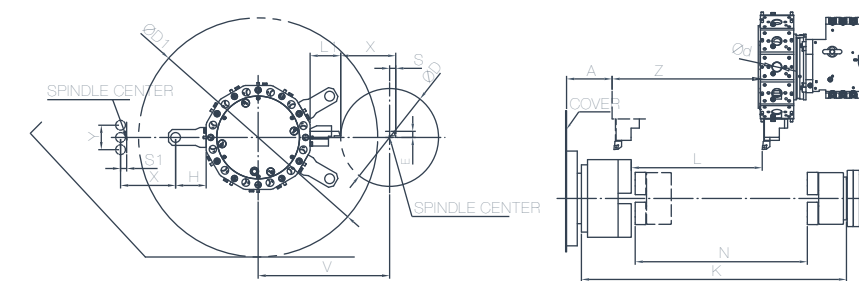
POWER TURRET / TWIN SPINDLE / SINGLE TURRET/ Y AXIS VDI RADIAL MOUNTING OPT.
