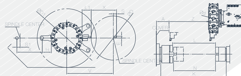
POWER TURRET / TWIN SPINDLE / SINGLE TURRET VDI RADIAL MOUNTING OPT.
