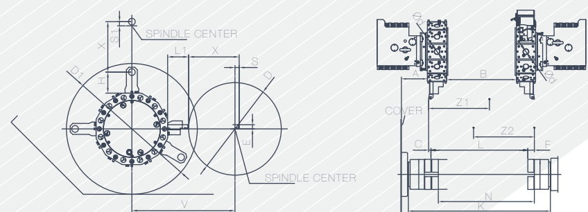
POWER TURRET / TWIN SPINDLE / TWIN TURRET VDI RADIAL MOUNTING OPT.
