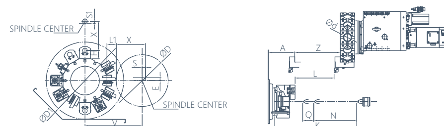
POWER TURRET BMT AXIAL MOUNTING OPT.
